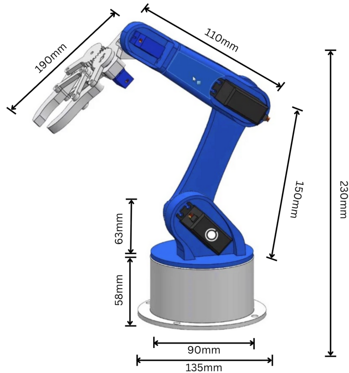
Figure 4.1: Robotic Arm
