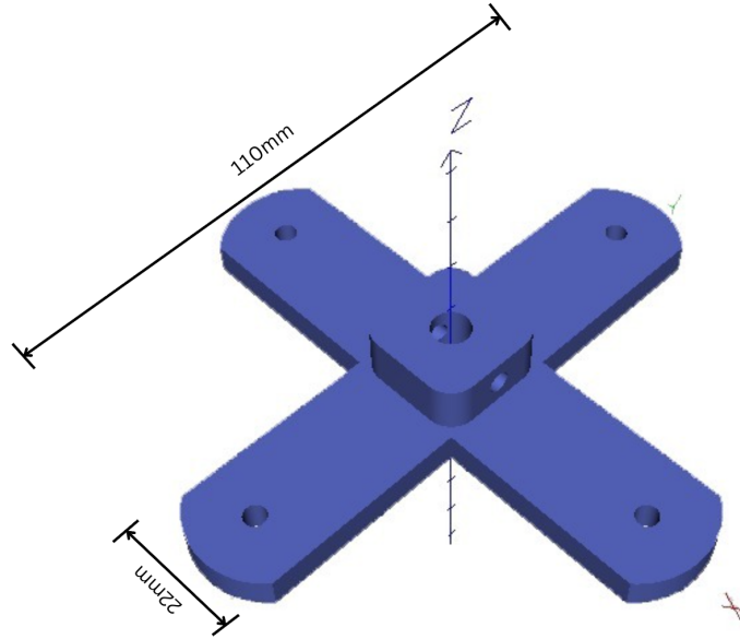
Figure 4.2: Robotic Arm
